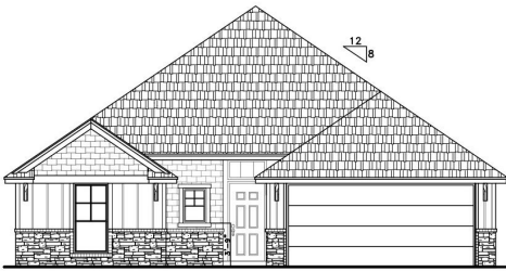
Elevation C
