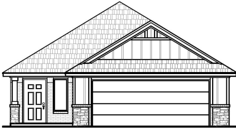
Elevation D
